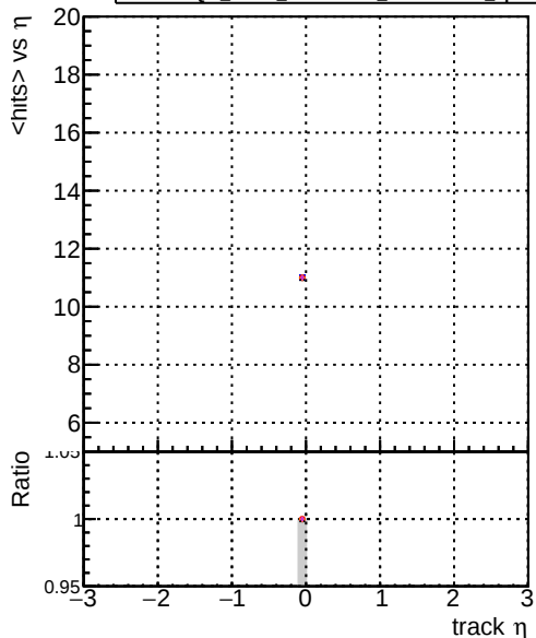
Legend for mean hits vs \eta : DOM mkFit XiMinusPU tetra and 2-lowpt DOM mkFit XiMinusPU NEWdefault specPless1-2-lowpt DOM mkFit XiMinusPU NEWdefault specPless2-2-lowpt DOM mkFit XiMinusPU NEWdefault specPless3-2-lowpt DOM mkFit XiMinusPU NEWdefault specPless4-2-lowpt
