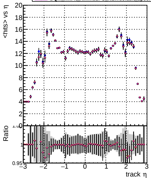
Legend for mean hits vs \eta : DOM mkFit XiMinusPU tetaIn2-lowpt DOM mkFit XiMinusPU NEWdefault specPless1-2-lowpt DOM mkFit XiMinusPU NEWdefault specPless2-2-lowpt DOM mkFit XiMinusPU NEWdefault specPless3-2-lowpt DOM mkFit XiMinusPU NEWdefault specPless4-2-lowpt
