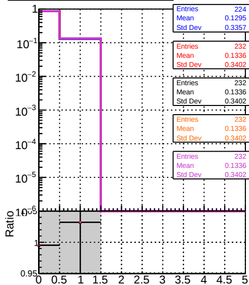
Legend for mean hits vs \eta : DOM mkFit XiMinusPU tetraaz2-lowpt DOM mkFit XiMinusPU NEWdefault specPless1-2-lowpt DOM mkFit XiMinusPU NEWdefault specPless2-2-lowpt DOM mkFit XiMinusPU NEWdefault specPless3-2-lowpt DOM mkFit XiMinusPU NEWdefault specPless4-2-lowpt
