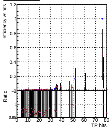
DOM_mkFit_XiMinusPU_retrain2-lowpt DOM_mkFit_XiMinusPU_NEWdefault_specPLess1-2-lowpt DOM_mkFit_XiMinusPU_NEWdefault_specPLess2-2-lowpt DOM_mkFit_XiMinusPU_NEWdefault_specPLess3-2-lowpt DOM_mkFit_XiMinusPU_NEWdefault_specPLess4-2-lowpt
