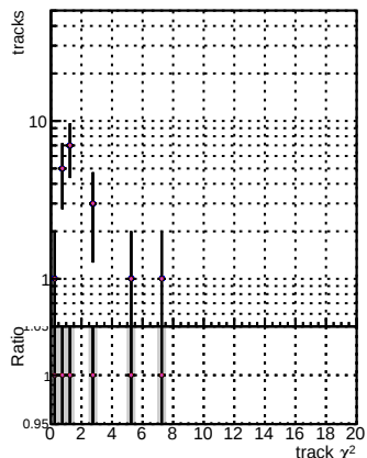
N of reco track vs. \chi^2 for different track classes
