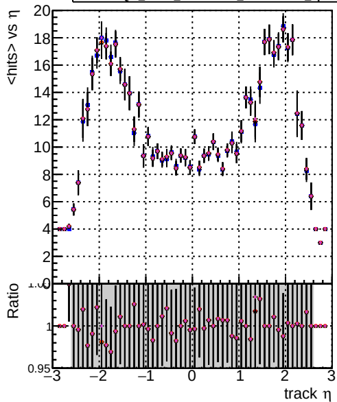
mean hit DOM mkFit XiMinusPU tetra2-lowpt specPless1-2-lowpt DOM mkFit XiMinusPU NEWdefault specPless1-2-lowpt DOM mkFit XiMinusPU NEWdefault specPless2-2-lowpt DOM mkFit XiMinusPU NEWdefault specPless3-2-lowpt DOM mkFit XiMinusPU NEWdefault specPless4-2-lowpt
