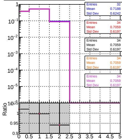
Legend: DOM mkFit XiMinusPU tetrax2-lowpt, DOM mkFit XiMinusPU NEWdefault specPless1-2-lowpt, DOM mkFit XiMinusPU NEWdefault specPless2-2-lowpt, DOM mkFit XiMinusPU NEWdefault specPless3-2-lowpt, DOM mkFit XiMinusPU NEWdefault specPless4-2-lowpt
