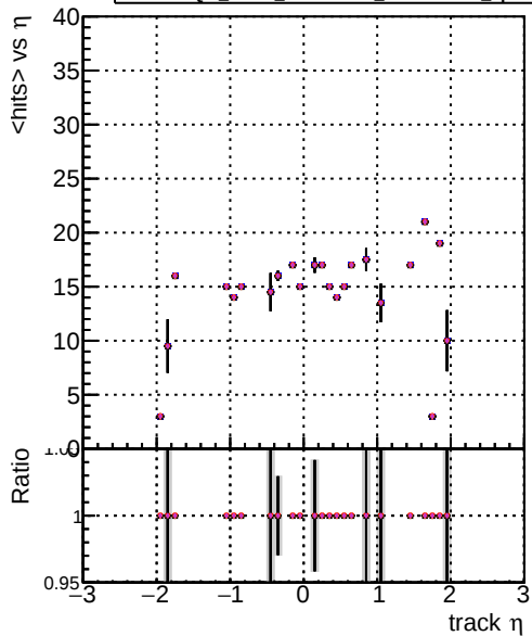
Legend: DOM mkFit XiMinusPU tetrax2-lowpt, DOM mkFit XiMinusPU NEWdefault specPless1-2-lowpt, DOM mkFit XiMinusPU NEWdefault specPless2-2-lowpt, DOM mkFit XiMinusPU NEWdefault specPless3-2-lowpt, DOM mkFit XiMinusPU NEWdefault specPless4-2-lowpt
