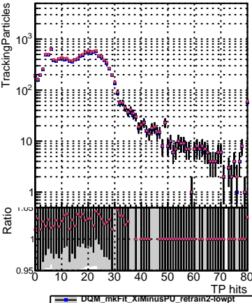
N of sim — DQM_mkFit_XiMinusPU_retrain2-lowpt — DQM_mkFit_XiMinusPU_NEWdefault_specPless1-2-lowpt — DQM_mkFit_XiMinusPU_NEWdefault_specPless2-2-lowpt — DQM_mkFit_XiMinusPU_NEWdefault_specPless3-2-lowpt — DQM_mkFit_XiMinusPU_NEWdefault_specPless4-2-lowpt
