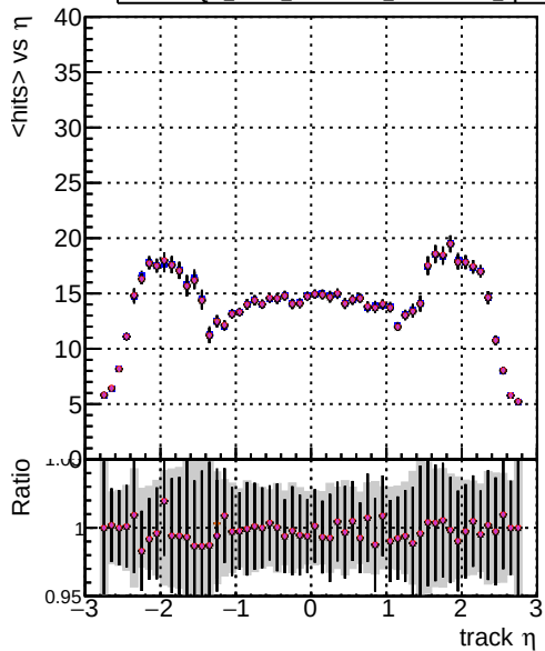
mean hit DOM mkFit XiMinusPU NEWdefault specPLess1-2-lowpt DOM mkFit XiMinusPU NEWdefault specPLess2-2-lowpt DOM mkFit XiMinusPU NEWdefault specPLess3-2-lowpt DOM mkFit XiMinusPU NEWdefault specPLess4-2-lowpt
