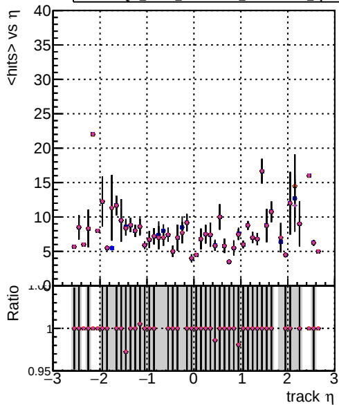
DOM mkFit XiMinusPU tetraaz2-lowpt specPLess1-2-lowpt DOM mkFit XiMinusPU NEWdefault specPLess1-2-lowpt DOM mkFit XiMinusPU NEWdefault specPLess3-2-lowpt DOM mkFit XiMinusPU NEWdefault specPLess3-2-lowpt DOM mkFit XiMinusPU NEWdefault specPLess4-2-lowpt
