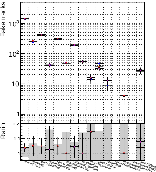
Number DOM_mkFit_XiMinusPU_NEWdefault_specPLess2-2-lowpt DOM_mkFit_XiMinusPU_NEWdefault_specPLess3-2-lowpt DOM_mkFit_XiMinusPU_NEWdefault_specPLess4-2-lowpt
