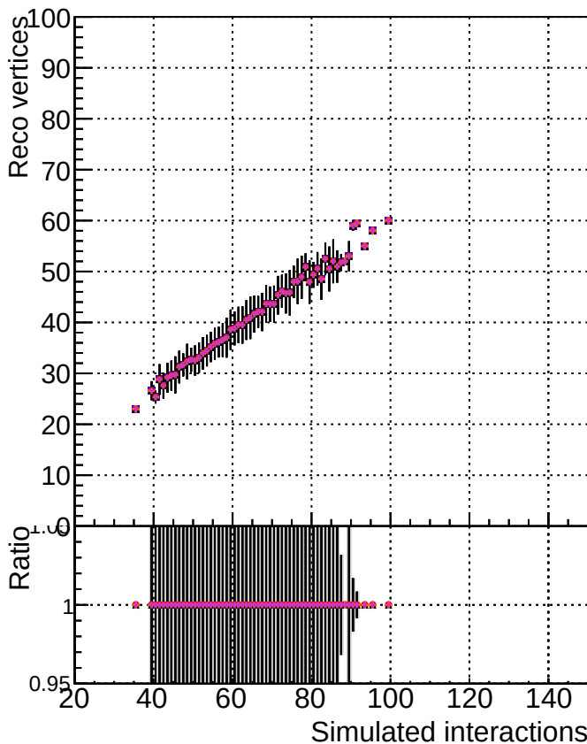
RecoVtx_vs_GenVtx
