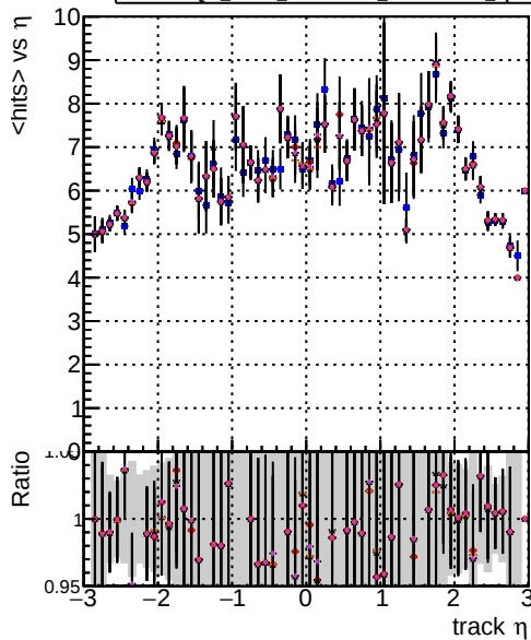
Legend for mean hits vs \eta : DOM mkFit XiMinusPU teta and 2-lowpt specPLess1-2-lowpt DOM mkFit XiMinusPU NEWdefault specPLess1-2-lowpt DOM mkFit XiMinusPU NEWdefault specPLess2-2-lowpt DOM mkFit XiMinusPU NEWdefault specPLess3-2-lowpt DOM mkFit XiMinusPU NEWdefault specPLess4-2-lowpt
