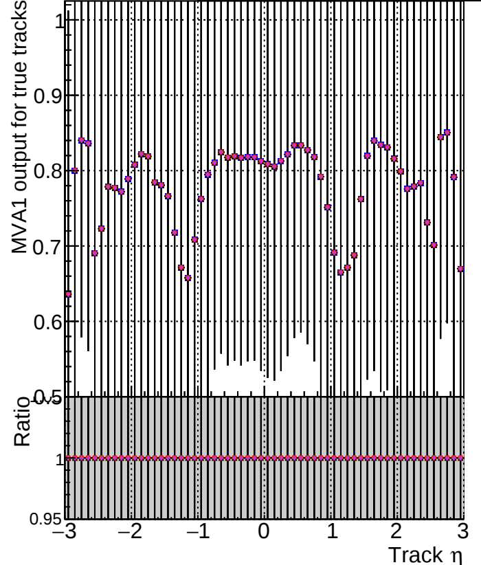
MVA1 of associated tracks (recoToSim) vs. track \eta Legend: DOM mkFit XiMinusPU retrain2-lowpt DOM mkFit XiMinusPU NEWdefault specPLess1-2-lowpt DOM mkFit XiMinusPU NEWdefault specPLess2-2-lowpt DOM mkFit XiMinusPU NEWdefault specPLess3-2-lowpt DOM mkFit XiMinusPU NEWdefault specPLess4-2-lowpt
