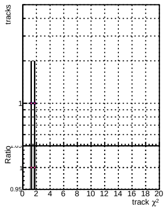
N of reco track vs. \chi^2 for different track selection criteria
