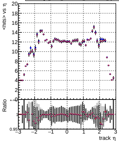
Legend for mean hits vs \eta : DOM mkFit XiMinusPU tetrano2-lowpt DOM mkFit XiMinusPU NEWdefault specLess1-2-lowpt DOM mkFit XiMinusPU NEWdefault specLess2-2-lowpt DOM mkFit XiMinusPU NEWdefault specLess3-2-lowpt DOM mkFit XiMinusPU NEWdefault specLess4-2-lowpt
