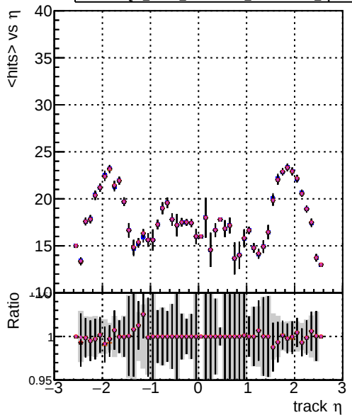
Legend for mean hits vs \eta : DOM mkFit XiMinusPU tetrain2-lowpt DOM mkFit XiMinusPU NEWdefault specPless1-2-lowpt DOM mkFit XiMinusPU NEWdefault specPless2-2-lowpt DOM mkFit XiMinusPU NEWdefault specPless3-2-lowpt DOM mkFit XiMinusPU NEWdefault specPless4-2-lowpt
