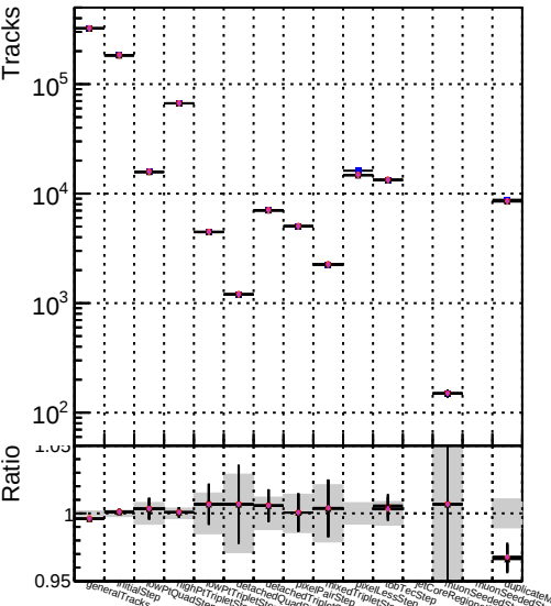
DOM mkFit XiMinusNOPU newDefault5 DOM mkFit XiMinusNOPU NEWdefault
