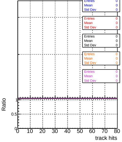
mean hit Legend: Blue line: DQM mkFit XiMinusNOPU NEWdefault specPless1 Red line: DQM mkFit XiMinusNOPU NEWdefault specPless3 Orange line: DQM mkFit XiMinusNOPU NEWdefault specPless3 Purple line: DQM mkFit XiMinusNOPU NEWdefault specPless4
