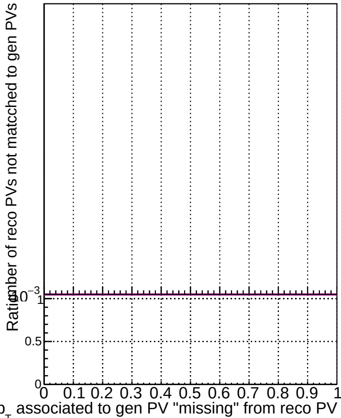
RecoPVAssoc2GenPVNotMatched_missing
