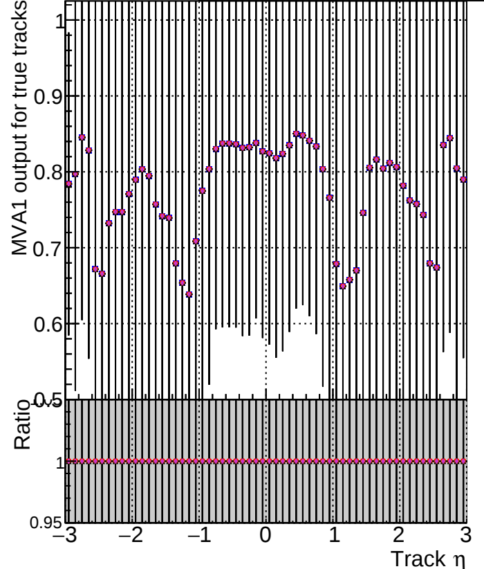
MVA1 of associated tracks (recoToSim) vs. track \eta Legend: DOM mkFit XiMinusNOPU newDefault5 DOM mkFit XiMinusNOPU NEWdefault specPless1 DOM mkFit XiMinusNOPU NEWdefault specPless2 DOM mkFit XiMinusNOPU NEWdefault specPless3 DOM mkFit XiMinusNOPU NEWdefault specPless4
