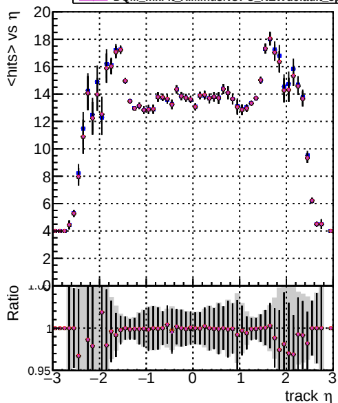
mean hits DOM mkFit XiMinusNOPU NEWdefault specPless1 DOM mkFit XiMinusNOPU NEWdefault specPless3 DOM mkFit XiMinusNOPU NEWdefault specPless3 DOM mkFit XiMinusNOPU NEWdefault specPless4
