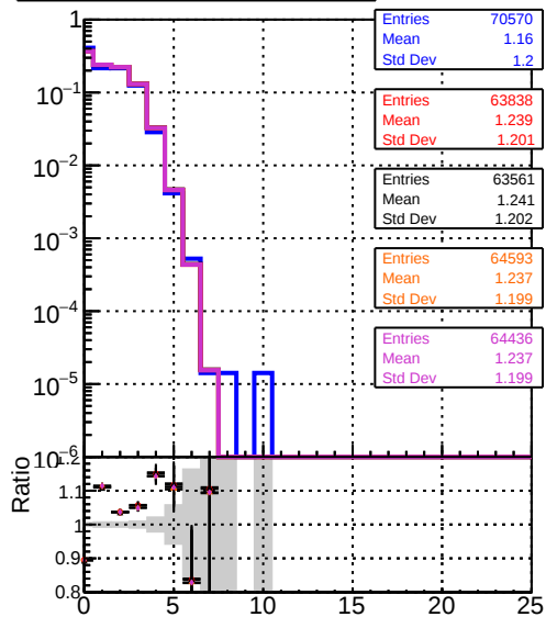
mean hits DOM mkFit XiMinusNOPU NEWdefault specPless1 DOM mkFit XiMinusNOPU NEWdefault specPless3 DOM mkFit XiMinusNOPU NEWdefault specPless4
