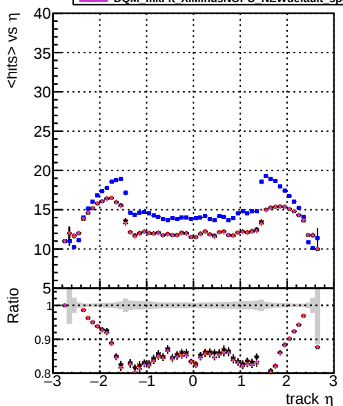
mean hits DOM mkFit XiMinusNOPU NEWdefault specPless1 DOM mkFit XiMinusNOPU NEWdefault specPless3 DOM mkFit XiMinusNOPU NEWdefault specPless4
