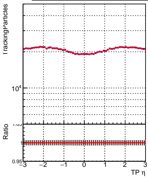
N of simulated tracks vs \eta DQM_mkFit_XiMinusNOPU_newDefault5 DQM_mkFit_XiMinusNOPUold-lowpt
