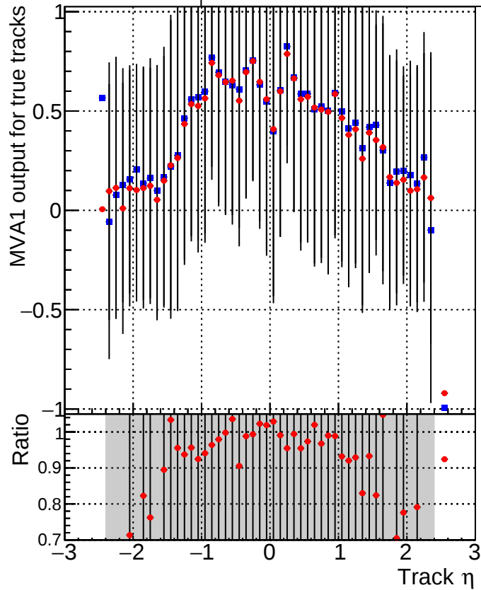
MVA1 of associated tracks (recoToSim) vs. track \eta Legend: ■ DQM_mkFit_XiMinusNOPU_newDefault5 ● DQM_mkFit_XiMinusNOPUold-lowpt
