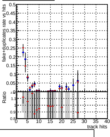
fake+duplicates vs hits
