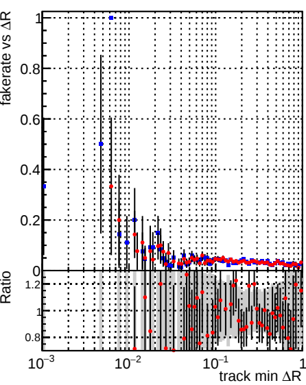
Legend: DQM_mkFit_XiMinusNOPU_newDefault5 (blue line with dots), DQM_mkFit_XiMinusNOPUold-lowpt (red line with dots)
