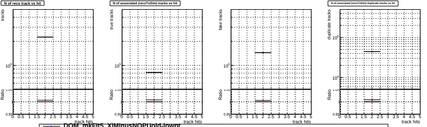
N of reco track vs hit N of associated (recoToSim) tracks vs hit fake tracks N of associated (recoToSim) duplicate tracks vs hit DQM_mkFit_XiMinusNOPU_old_lowpt DQM_mkFit_XiMinusNOPU_NEWdefault5 DQM_mkFit_XiMinusNOPU_NEWdefault5_specPLESS3
