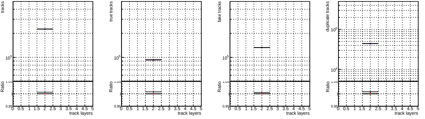
N of reco track vs hit N of associated (recoToSim) tracks vs hit fake tracks N of associated (recoToSim) duplicate tracks vs hit DQM_mkFit_XiMinusNOPU_old_lowpt DQM_mkFit_XiMinusNOPU_NEWdefault5 DQM_mkFit_XiMinusNOPU_NEWdefault5_specPLESS3
