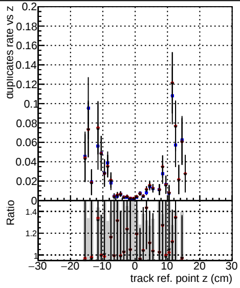
Legend: DQM_mkFit5_XiMinusNOPUold-lowpr (blue circles) DQM_mkFit5_XiMinusNOPUnewDefault5 (red circles) DQM_mkFit5_XiMinusNOPUnewDefault5_specPLess3 (black circles)
