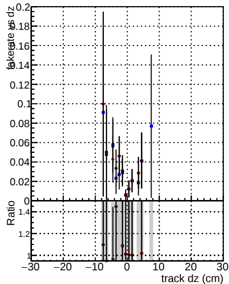
Fake rate vs dz Legend: DOM mkFit5 XiminusNOPUold-lowpt DOM mkFit5 XiminusNOPUold-highpt DOM mkFit5 XiminusNOPUnewDefault5 DOM mkFit5 XiminusNOPUnewDefault3 specPLeSS3
