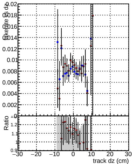
Fake rate vs dz DOM mkFit5 XiMinusNOPUold-lowpt DOM mkFit5 XiMinusNOPUold-highpt DOM mkFit5 XiMinusNOPUnewPUL5 DOM mkFit5 XiMinusNOPUnewdefault specPLess3
