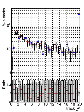
N of reco track vs. DGM mrFit XiMinus NPU old (top) DGM mrFit XiMinus NPU new default5 DGM mrFit XiMinus NPU new default specPLess3
