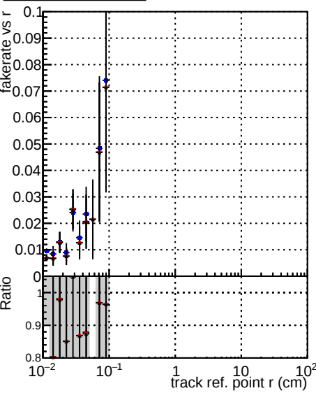
Legend: DQM_mkFit5_XiMinusNOPUold-lowpt (blue dots) DQM_mkFit5_XiMinusNOPUnewDefault5 (red dots) DQM_mkFit5_XiMinusNOPUnewDefault5_specPLess3 (black dots)
