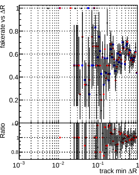
Legend: DQM_mkFit5_XiMinusNOPUold-lowpt (blue dots), DQM_mkFit5_XiMinusNOPU_newDefault5 (red dots), DQM_mkFit5_XiMinusNOPU_NEWdefault_specPLess3 (black dots with error bars)
