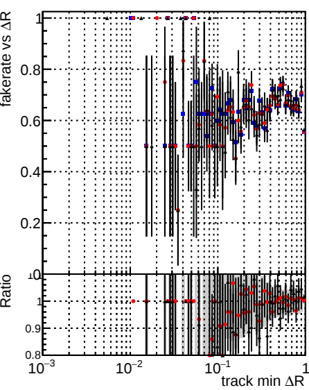
Legend: DQM_mkFit5_XiMinusNOPUold-lowpr (blue), DQM_mkFit5_XiMinusNOPU_newDefault5 (red), DQM_mkFit5_XiMinusNOPU_NEWdefault_specPLess3 (black)
