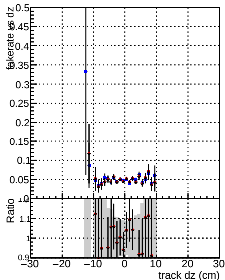
Fake rate vs dz Legend: DOM mkFit5 XiMinusNOPUold-lowpt DOM mkFit5 XiMinusNOPUnewDefault5 DOM mkFit5 XiMinusNOPUnewDefault5 specPLess3
