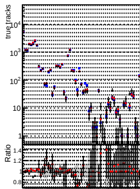
Legend: BOM mkFit5 XMinusNOPU old_lowpt (blue), BOM mkFit5 XMinusNOPU new_lowpt5 (red), BOM mkFit5 XMinusNOPU new_lowpt5 specPLess3 (black)
