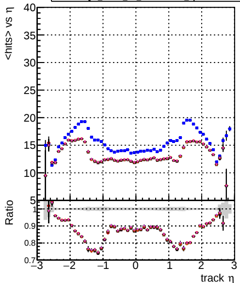
mean hits vs \eta DOM mkFit TT NEWdefault specPless1 DOM mkFit TT NEWdefault specPless2 DOM mkFit TT NEWdefault specPless3 DOM mkFit TT NEWdefault specPless4
