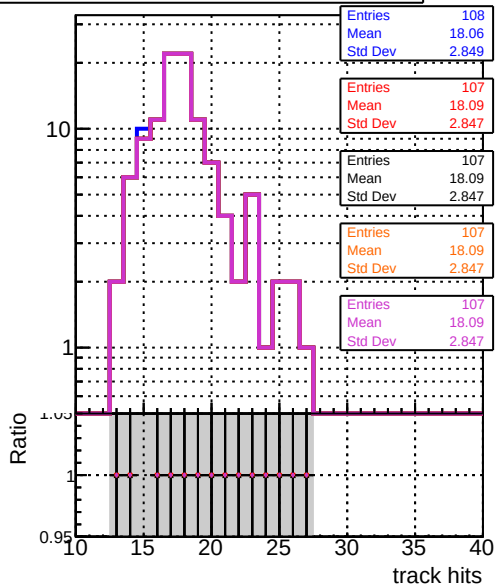
mean hit DOM mkFit TT (tdrw) NEWdefault specPless1 DOM mkFit TT (tdrw) NEWdefault specPless2 DOM mkFit TT (tdrw) NEWdefault specPless3 DOM mkFit TT (tdrw) NEWdefault specPless4
