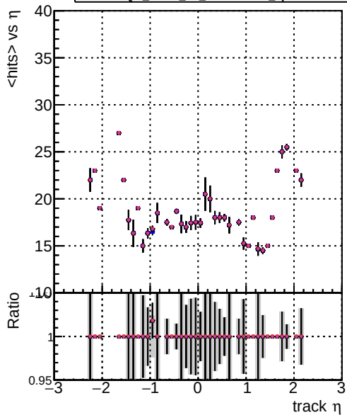
mean hit DOM mkFit TT (tdrw) NEWdefault specPless1 DOM mkFit TT (tdrw) NEWdefault specPless2 DOM mkFit TT (tdrw) NEWdefault specPless3 DOM mkFit TT (tdrw) NEWdefault specPless4
