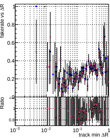
Fake rate vs \Delta R(\text{track, jet}) Legend: DOM (blue), mkt (red), fit (green), TT (black), retrain (purple), Newdata (orange), spec (grey), specLess1 (light grey), specLess2 (lighter grey), specLess3 (lightest grey).
