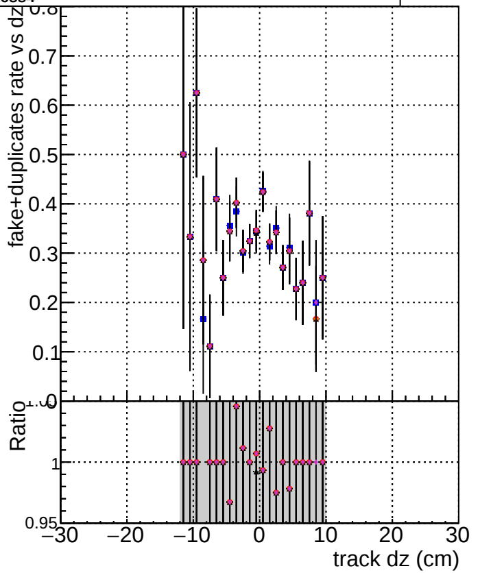
DQM_mkFit_TT_retrain DQM_mkFit_TT_NEWdefault_specPLess1 DQM_mkFit_TT_NEWdefault_specPLess2 DQM_mkFit_TT_NEWdefault_specPLess3 DQM_mkFit_TT_NEWdefault_specPLess4
