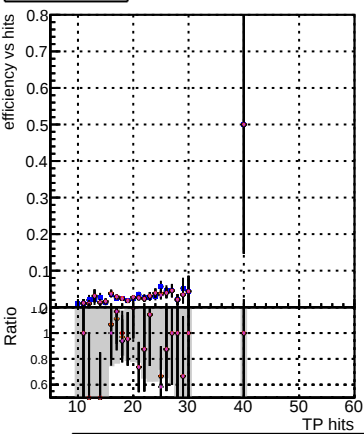
Efficiency vs TP hits Legend: DOM_mkFit_TT_retrain DOM_mkFit_TT_NEWdefault_specPless1 DOM_mkFit_TT_NEWdefault_specPless2 DOM_mkFit_TT_NEWdefault_specPless3 DOM_mkFit_TT_NEWdefault_specPless4
