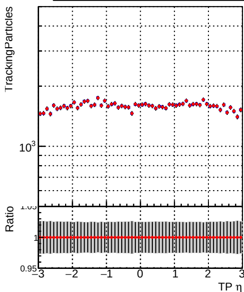
N of simulated tracks vs \eta N of associated tracks (simToReco) vs \eta
