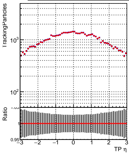
N of simulated tracks vs TP \eta — DQM_mkFit_TT_retrain — DQM_mkFit_TTold
