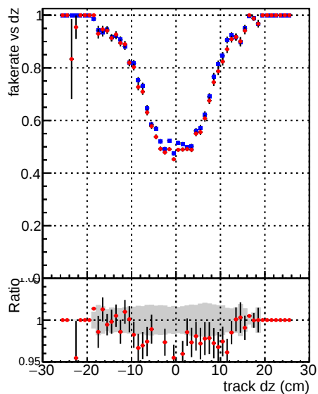
Fake rate vs dz — DQM_mkFit_TT_retrain — DQM_mkFit_TTold
