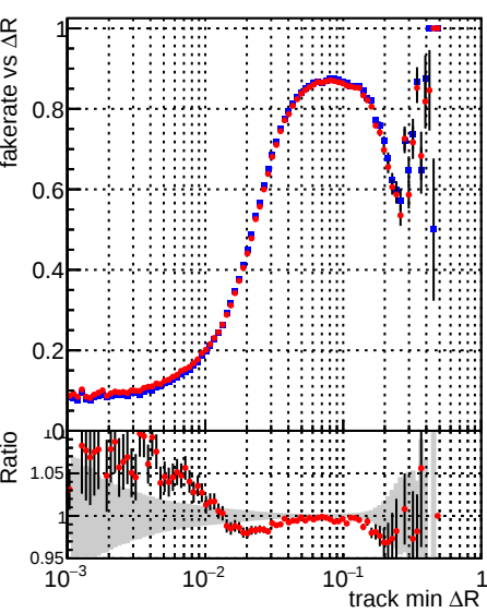
Fake rate vs \Delta R(\text{track, jet}) Legend: DQM_mkFit_TT_retrain (blue dots), DQM_mkFit_TTold (red dots)
