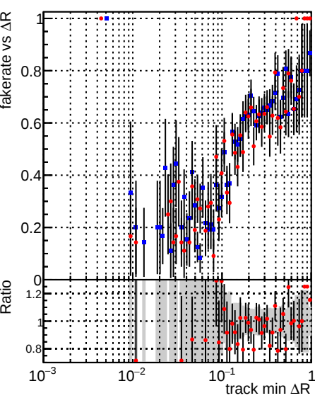
Fake rate vs \Delta R(\text{track, jet}) Legend: DQM_mkFit_TT_retrain (blue squares) DQM_mkFit_TTold (red circles)
