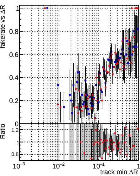
Fake rate vs \Delta R(\text{track, jet}) Legend: ■ DQM_mkFit_TT_retrain ● DQM_mkFit_TTold
