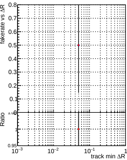
Fake rate vs \Delta R(\text{track, jet}) Legend: DQM_mkFit_TT_retrain (grey line with blue dots) DQM_mkFit_TTold (red line with red dots)
