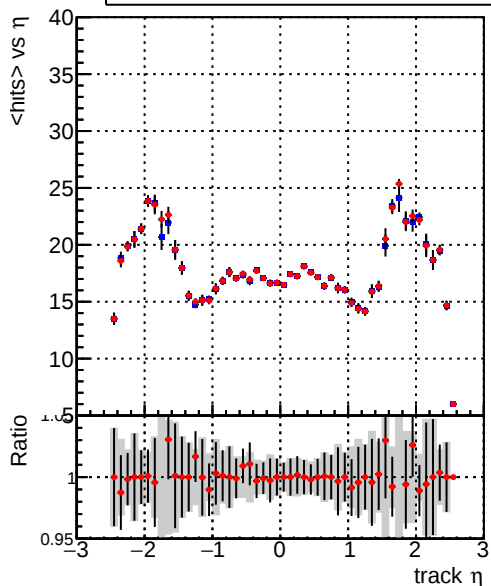
mean hits Legend: — DQM_mkFit_TT_retrain, — DQM_mkFit_TTold
